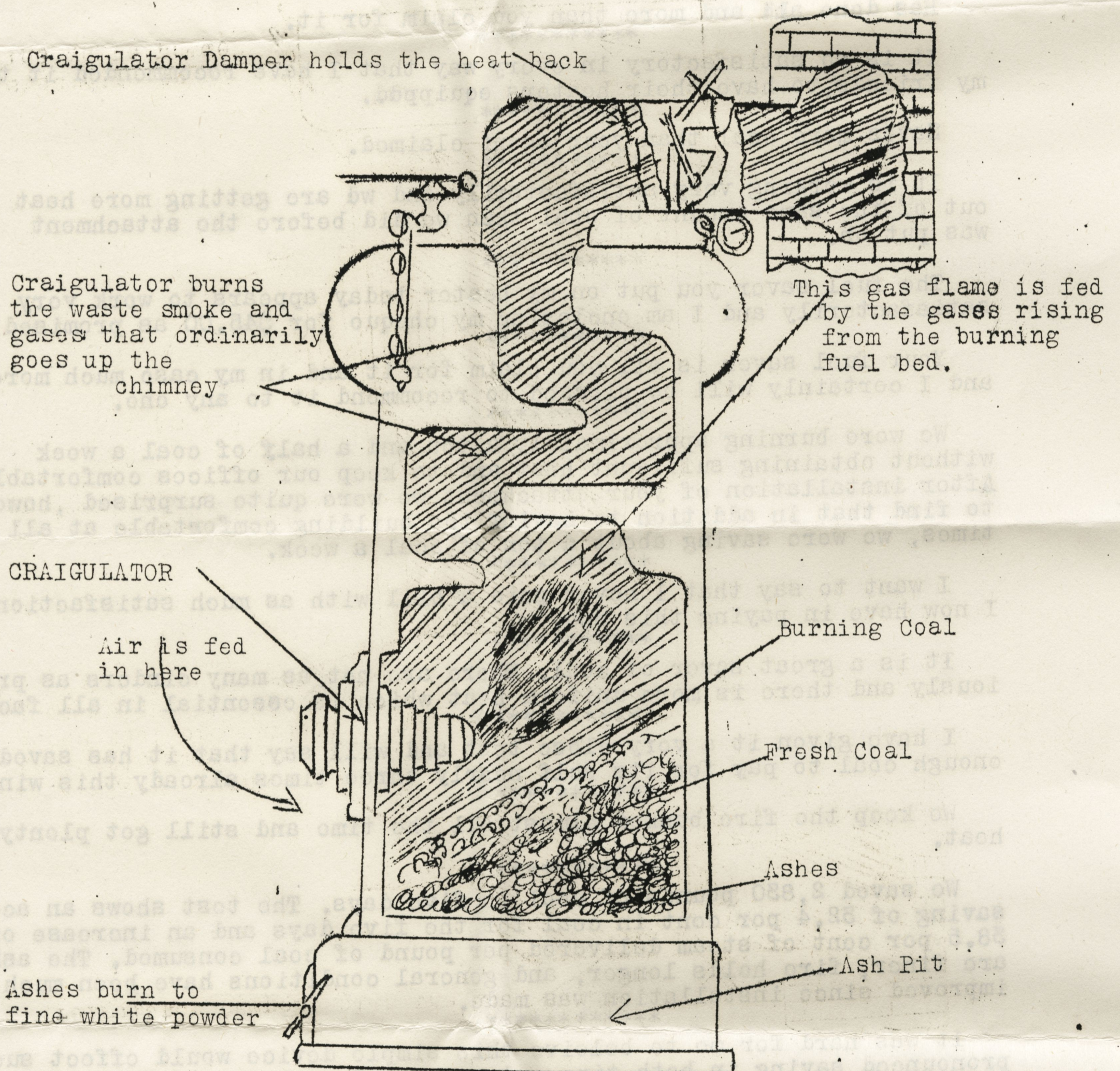
Furnace with CRAIGULATOR
